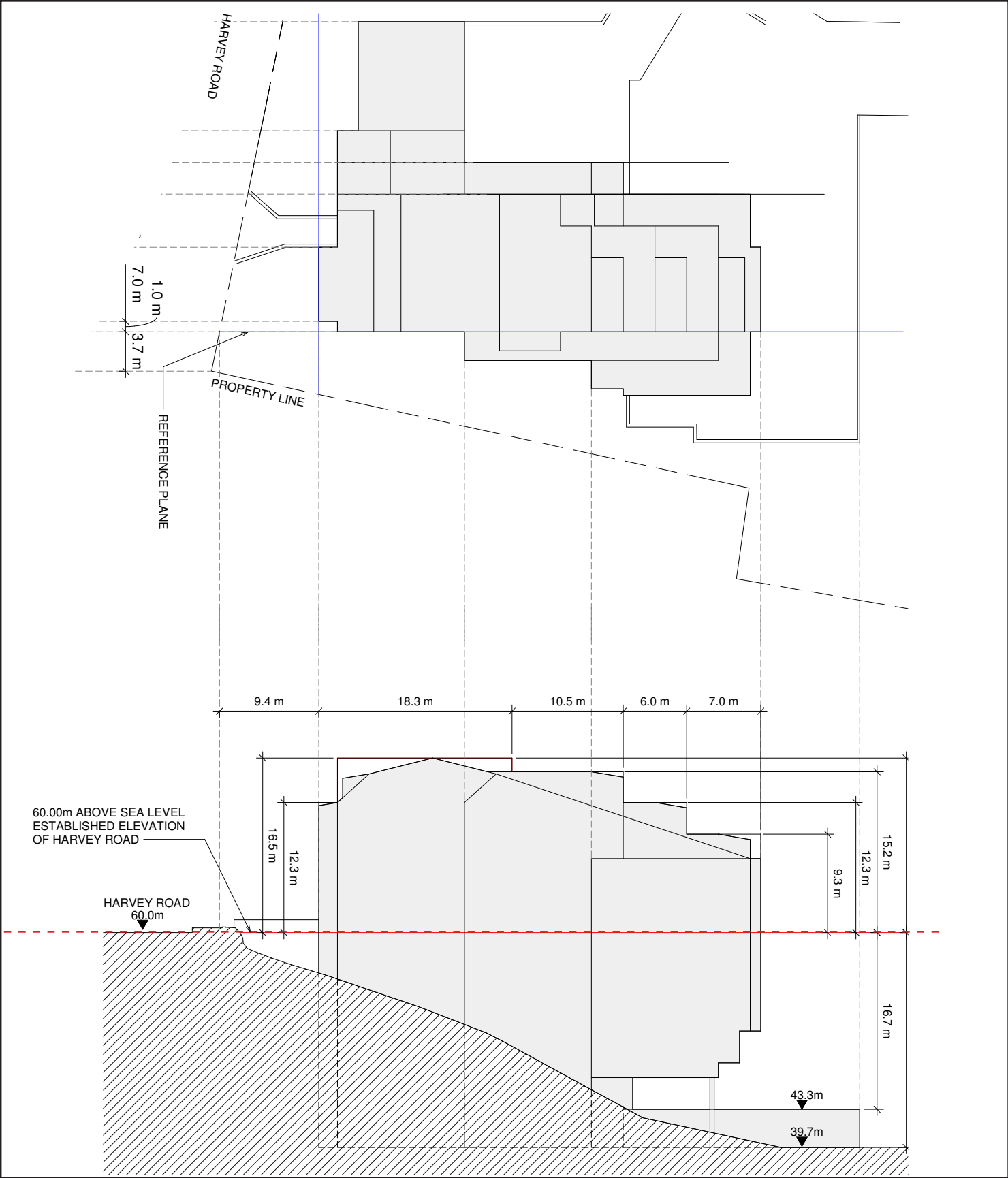
Figure C2: West Elevation
